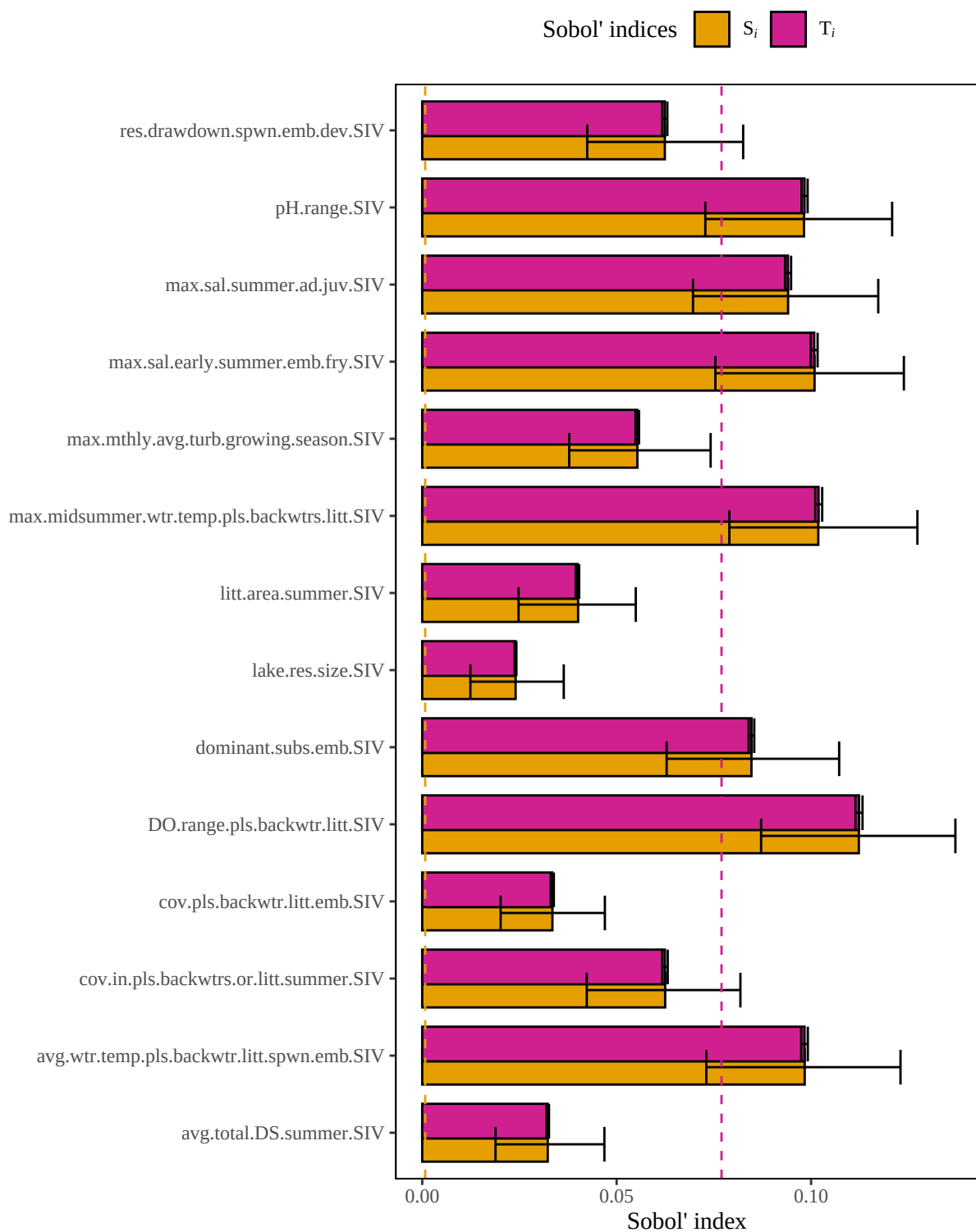
Figure 4. Results of a sensitivity analysis for the blackbullheadLac model based on an arithmetic mean structure. Dashed lines represent baseline numerical approximation error for S_i and T_i ( i.e. , dummy variables).
