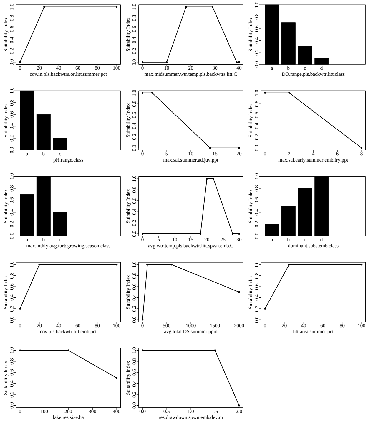
Figure 1. Suitability index graphs for variables included in the blackbullheadLac model in ecores.
